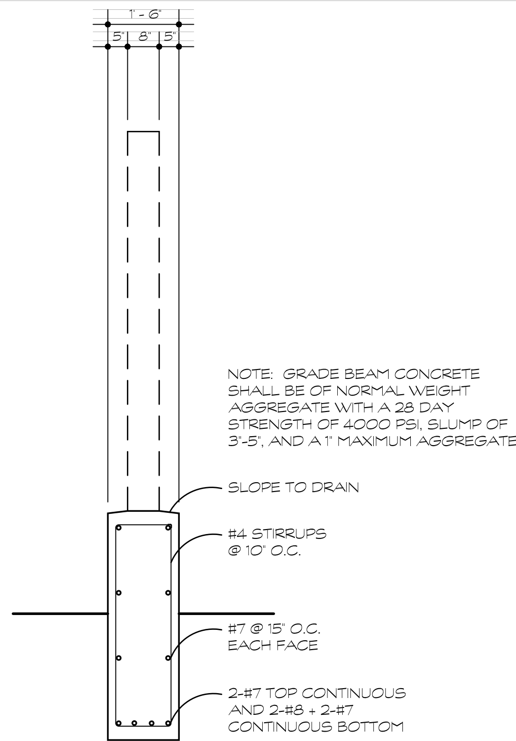
2 MONUMENT SIGN FOOTING
