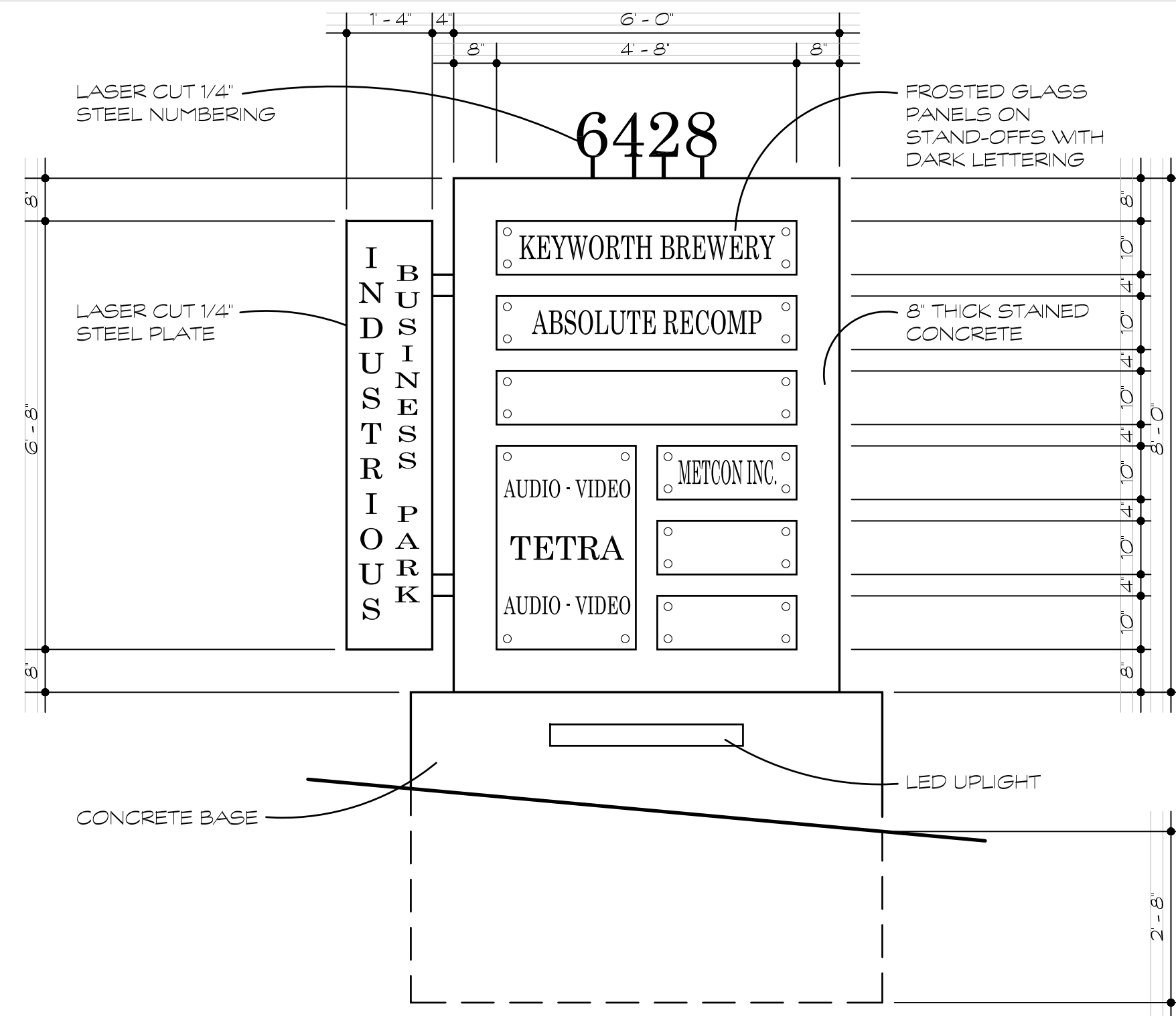
1 DOUBLE SIDED MONUMENT SIGN
