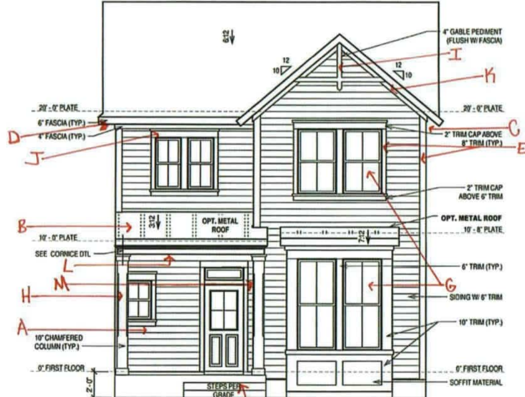
FRONT ELEVATION "B" (VICTORIAN)
