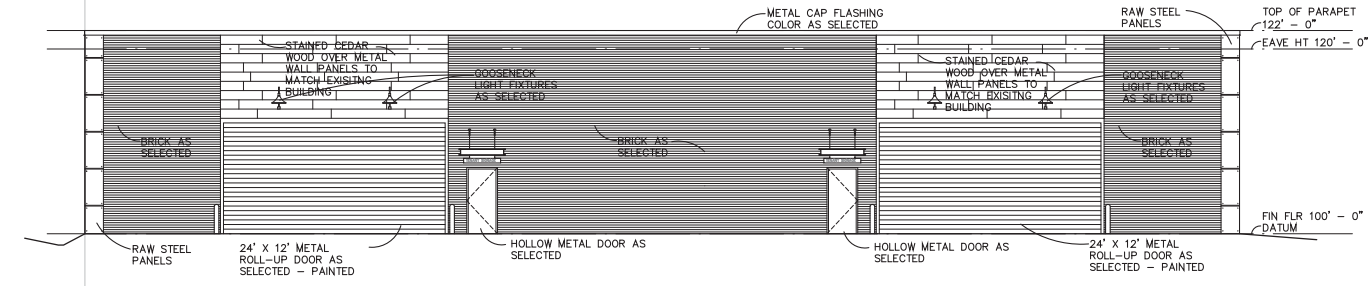
1 WEST EXTERIOR BUILDING ELEVATION 1/8" = 1' - 0"
