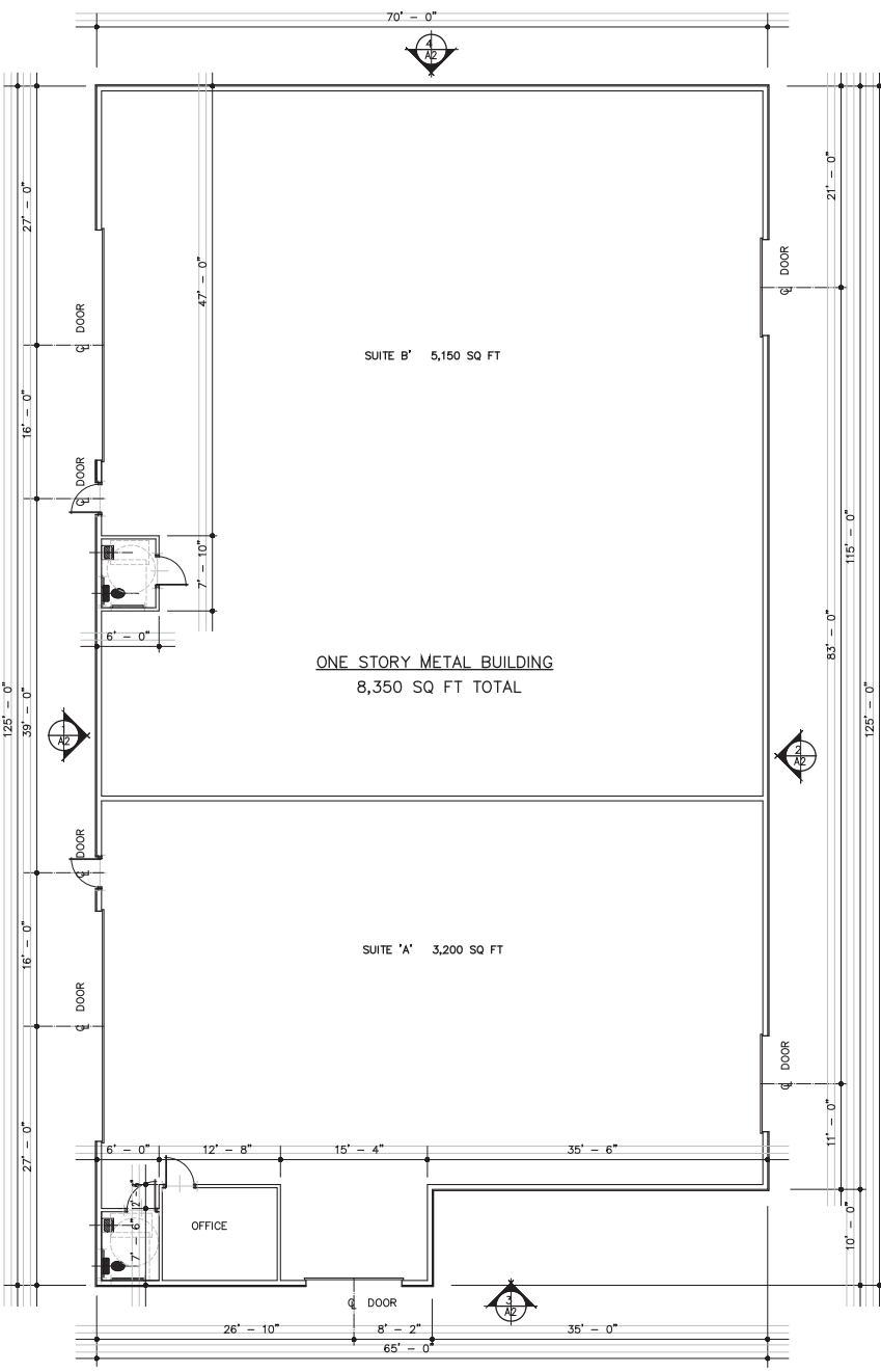
A OVERALL FLOOR PLAN BUILDING 'B' 1/8" = 1' - 0"
