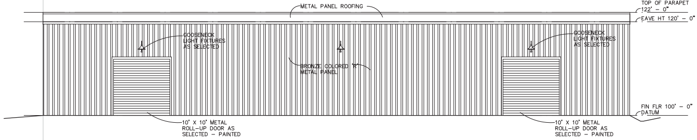
2 EAST EXTERIOR BUILDING ELEVATION 1/8" = 1' - 0"
