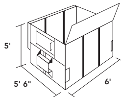
6-CUBIC-YARD LOW TOP AND END-LOADING
