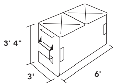
2-CUBIC-YARD
