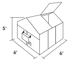
6-CUBIC-YARD SLANT
