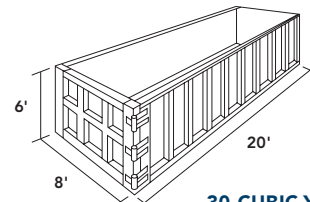
30-CUBIC-YARD
