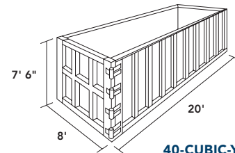
40-CUBIC-YARD
