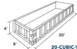
20-CUBIC-YARD
