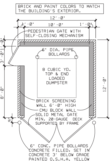
REFUSE CONTAINER PLAN VIEW (TYP.) N.T.S.
